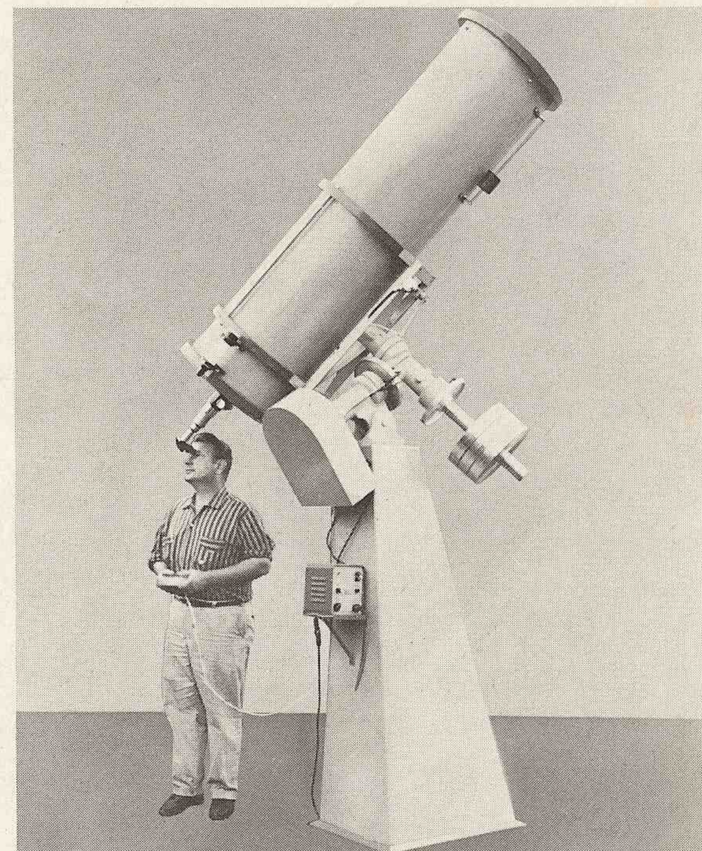
16" F/16 EFL CASSEGRAIN - Dall-Kirkham
