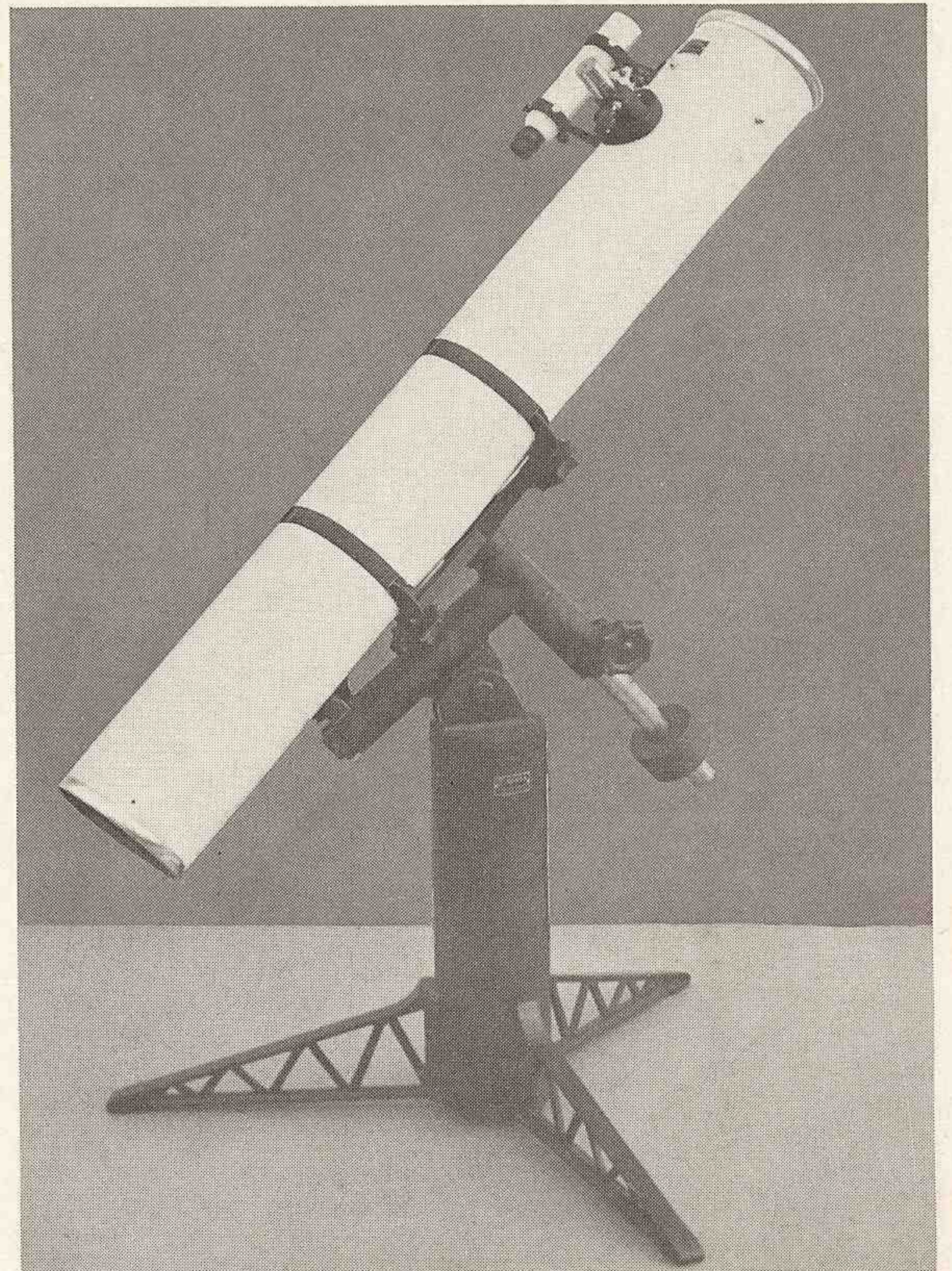
6" F/8 MODEL "A" STANDARD
