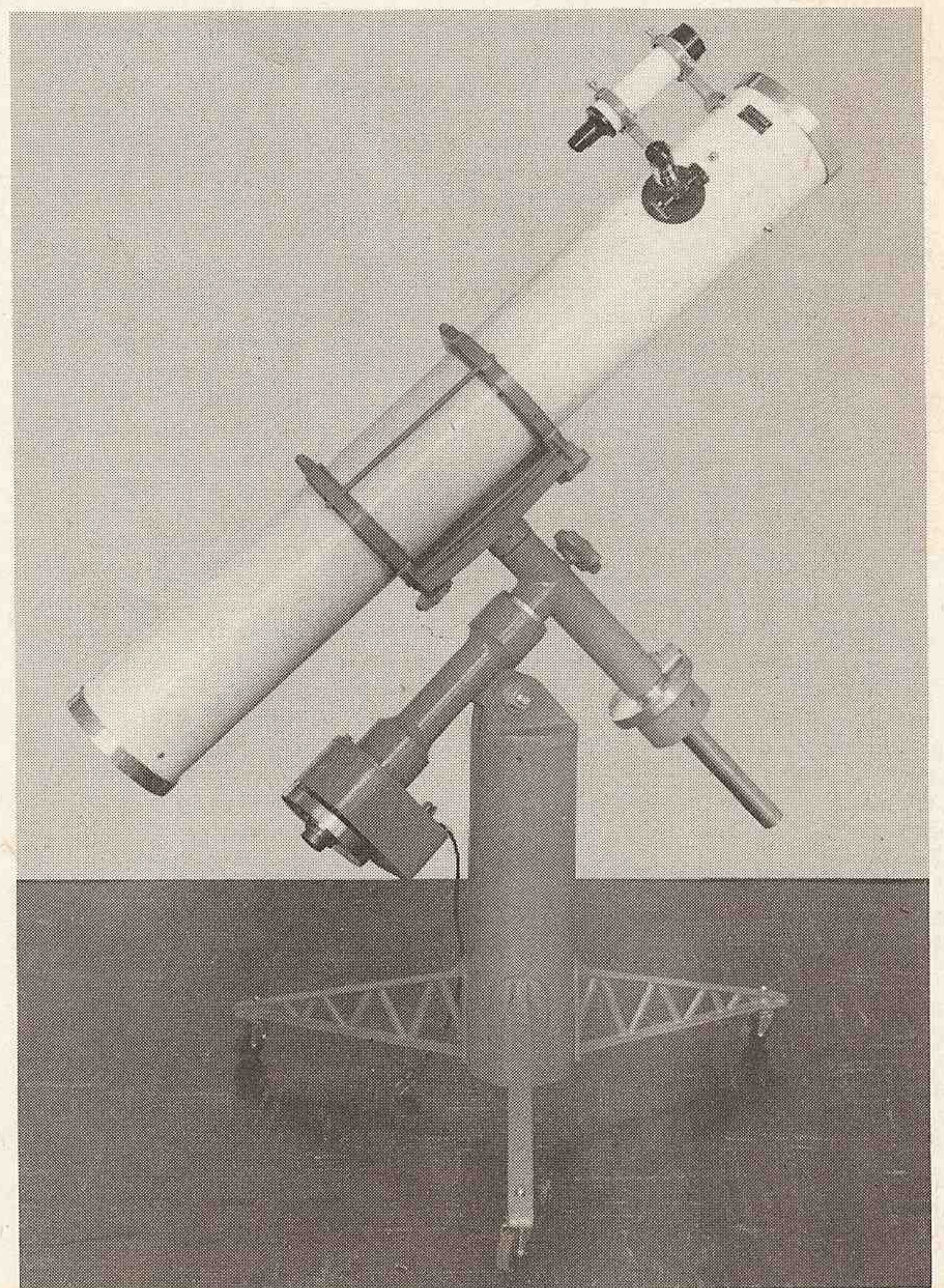
6" F/8 MODEL "A" DELUXE
