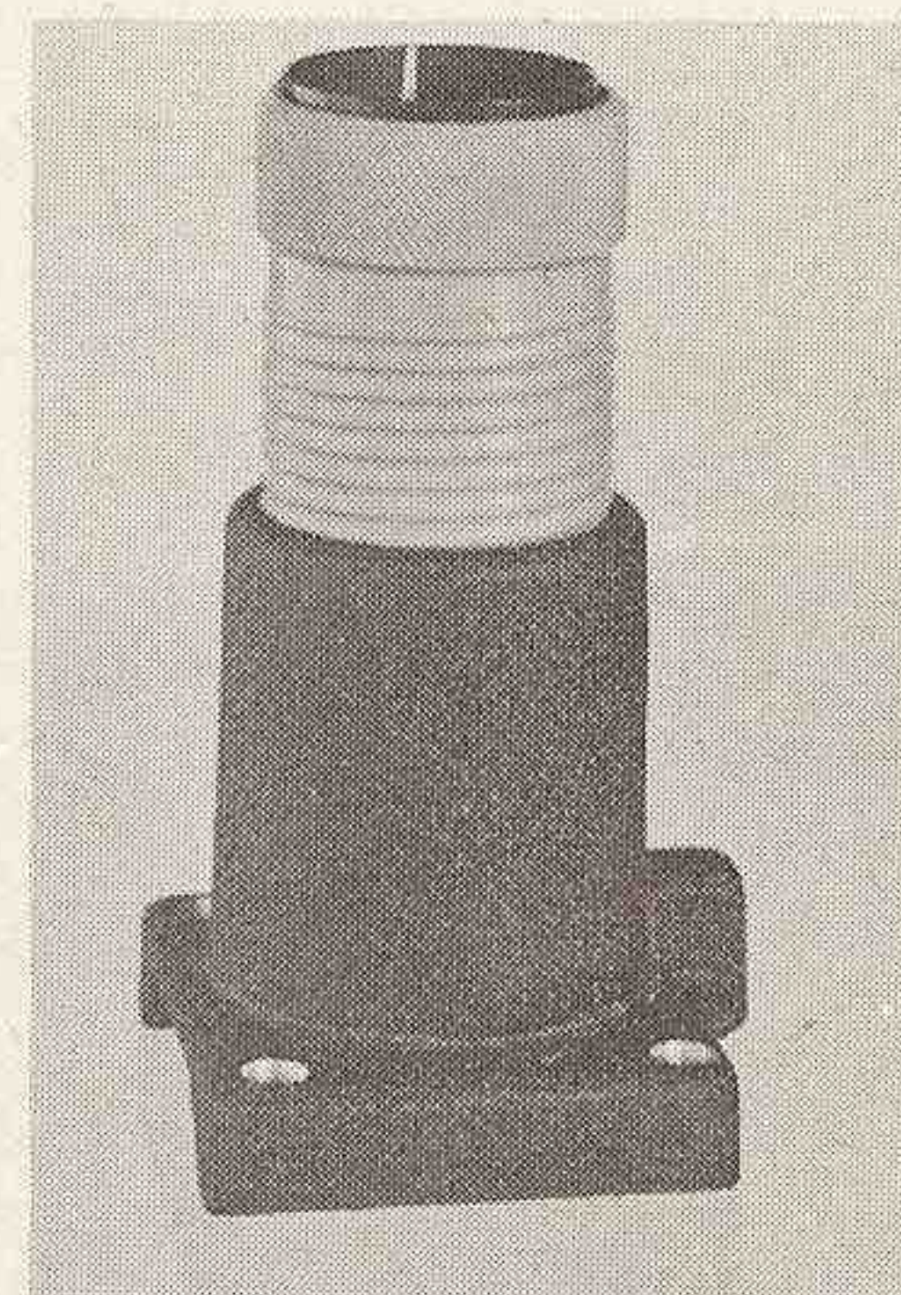
Angle Rack and Pinion focuser, 1¼" $27.50. Helical focuser $15.95. Rack and Pinion and Helical focuser combined $27.50 (when available)
