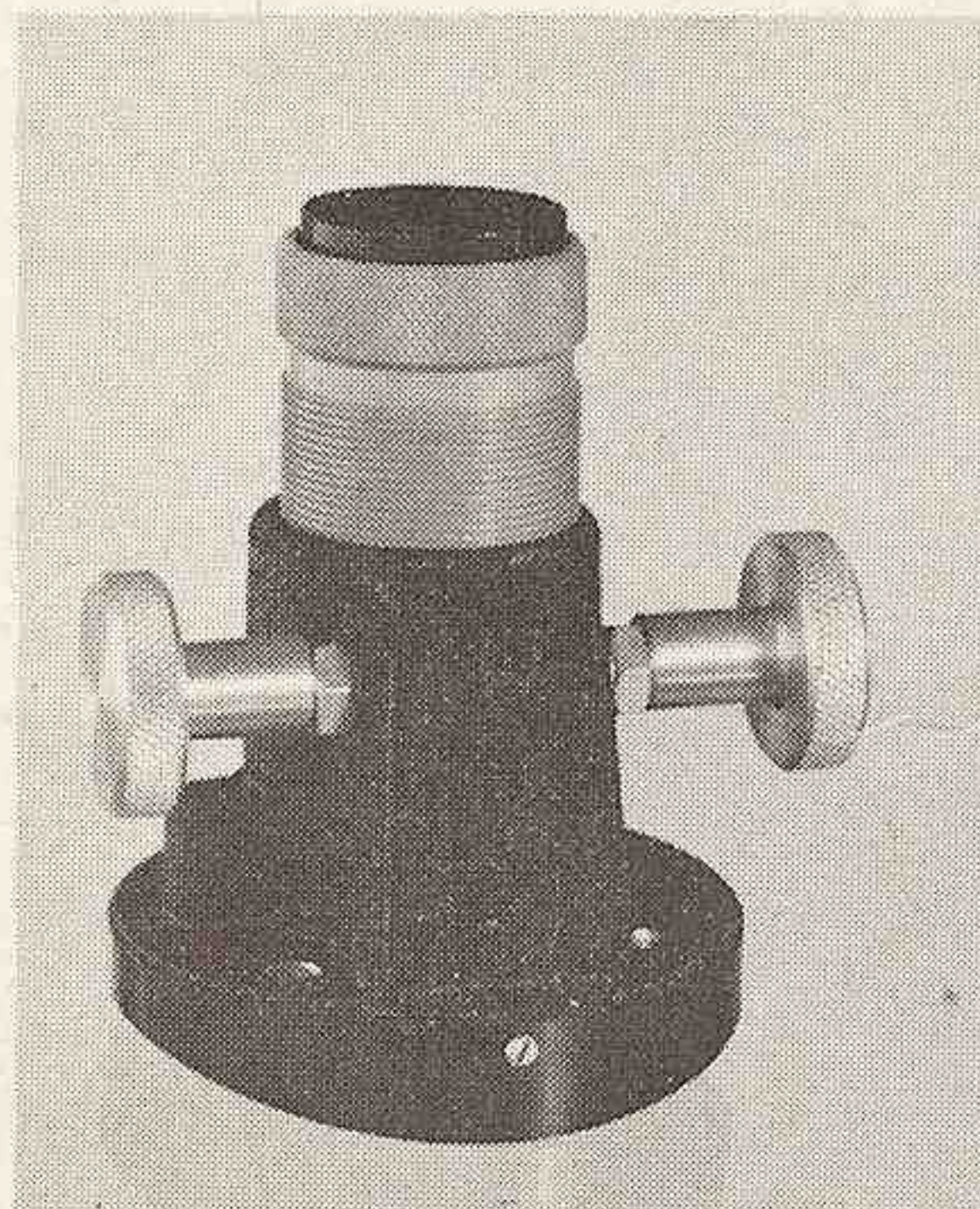
Angle Rack and Pinion focuser, 1¼" $27.50. Helical focuser $15.95. Rack and Pinion and Helical focuser combined $27.50 (when available)
