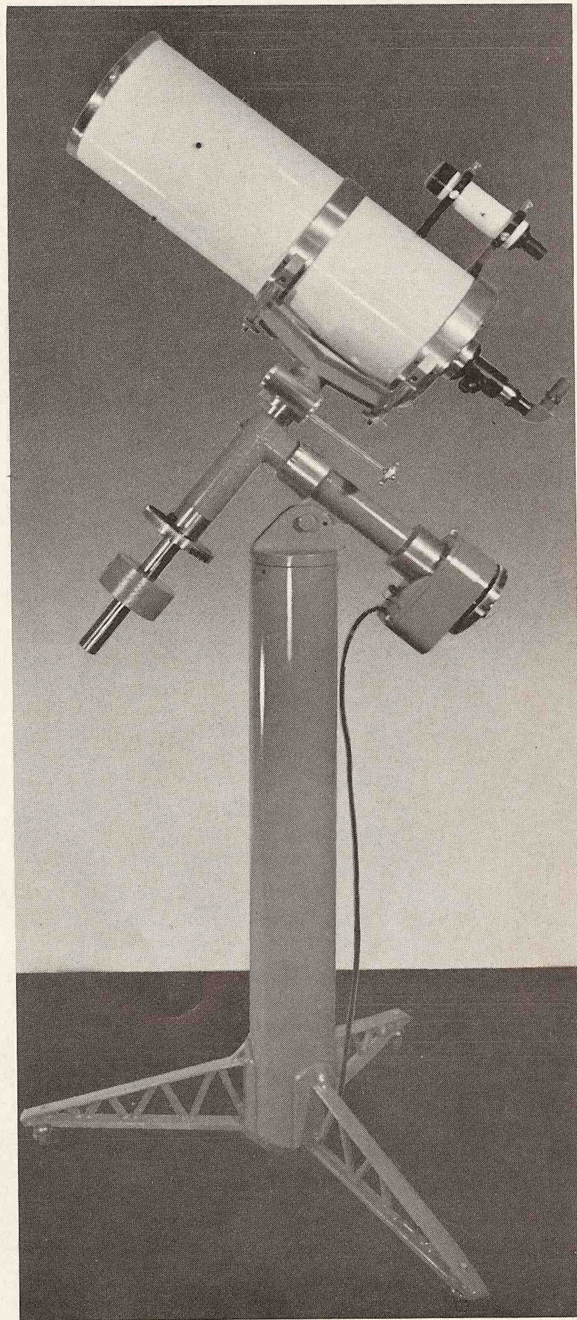
8" F/15 CASSEGRAIN
